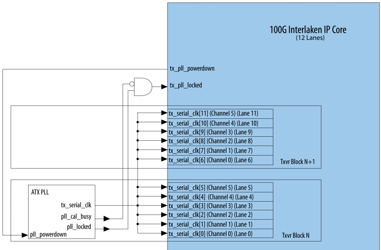
Figure 2-6: Example Connection of ATX PLL with 100G Interlaken IP Core Using Arria 10 xN Clock Network
