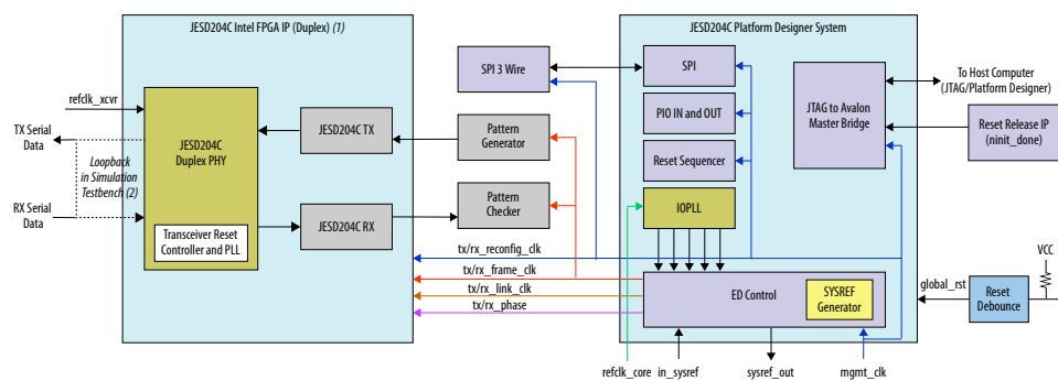
Figure 2. JESD204C Design Example High-level Block Diagram
