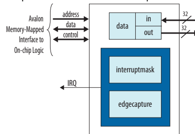
Figure 8. PIO Core with Input Ports, Output Ports, and IRQ Support
