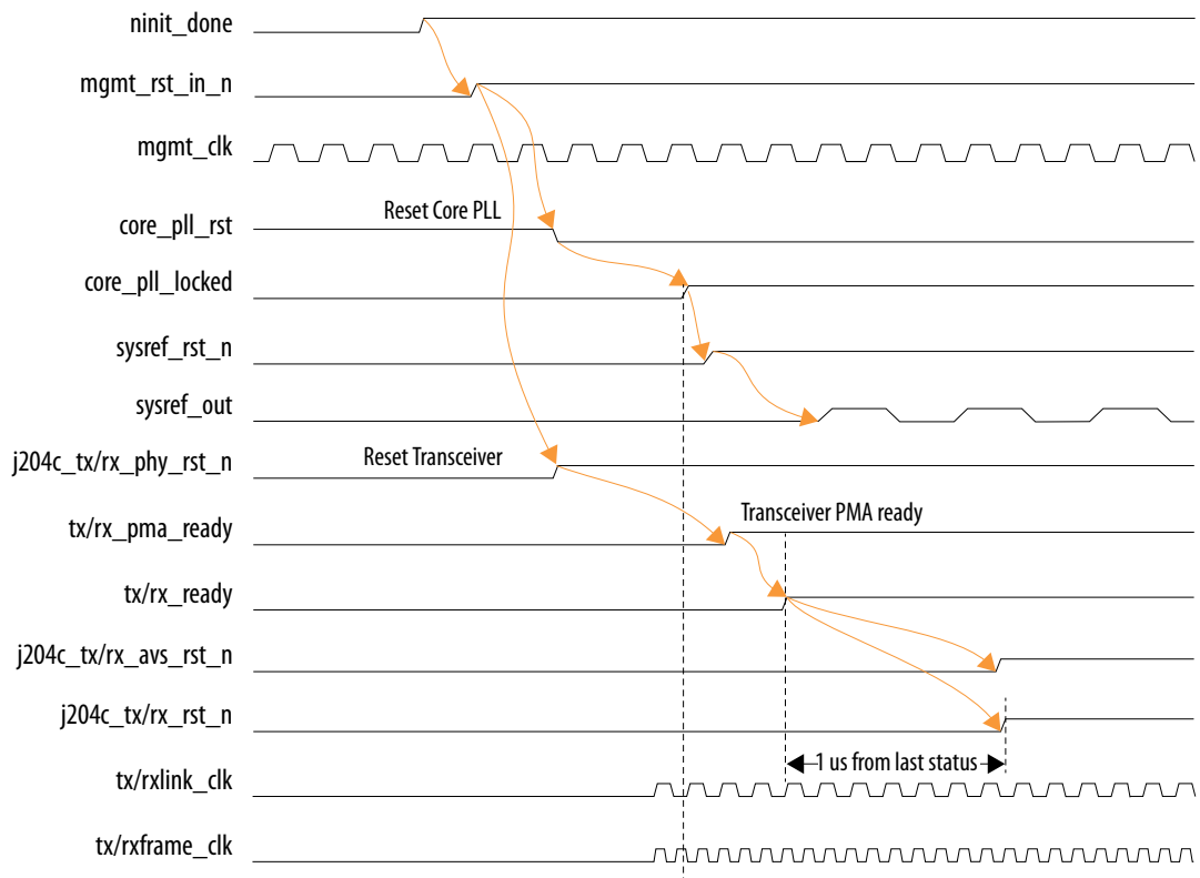
Figure 9. Timing Diagram for the Design Example Resets
