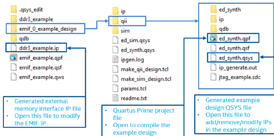
Figure 3. Generated Synthesizable Design Example File Structure
