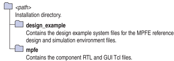
Figure 5. Directory Structure
