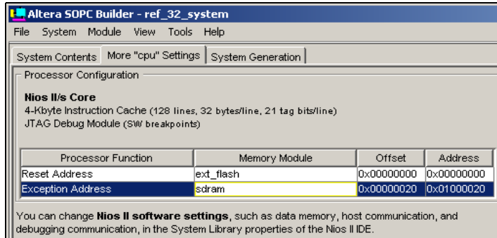
Figure 4-7. Nios II CPU Settings for Reset & Exception Locations
