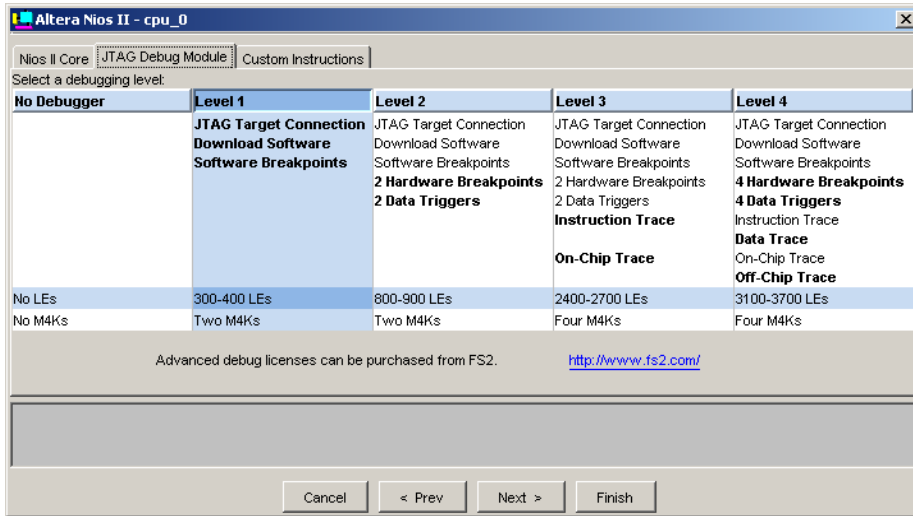
Figure 4–4. Nios II Wizard – Debug Configuration
