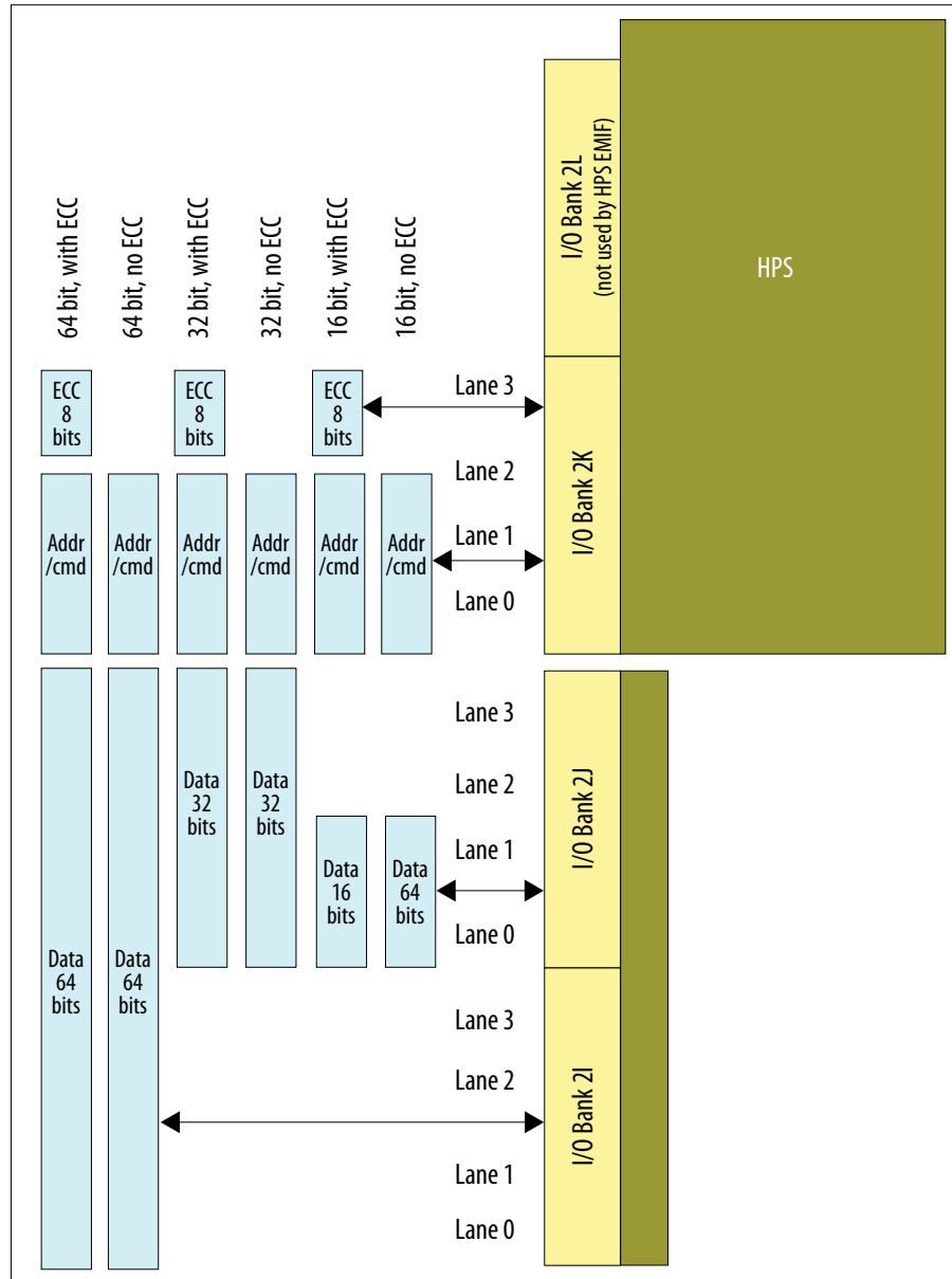
Figure 3. Intel Arria 10 SoC EMIF Pin Options
