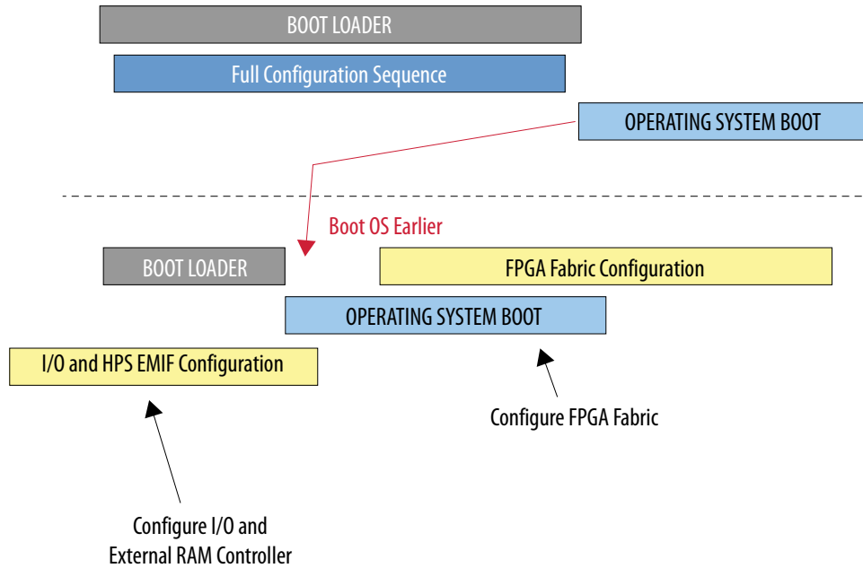
Figure 1. Early I/O Release
