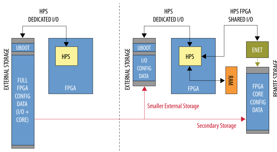
Figure 2. Early I/O Release allows FPGA fabric image to be accessed through a Shared I/O Interface
