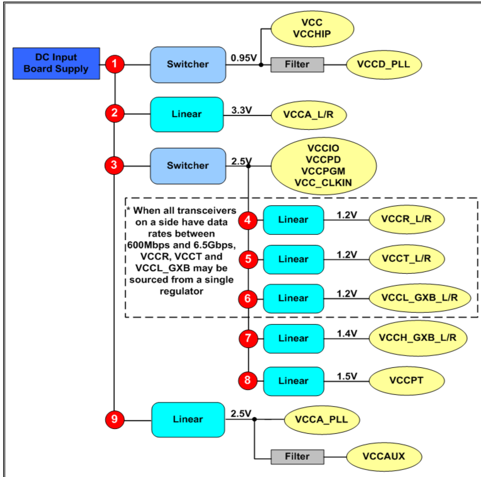
Figure 1. Example Stratix IV GT Power Supplies Block Diagram for Data Rates > 2.488 Gbps
